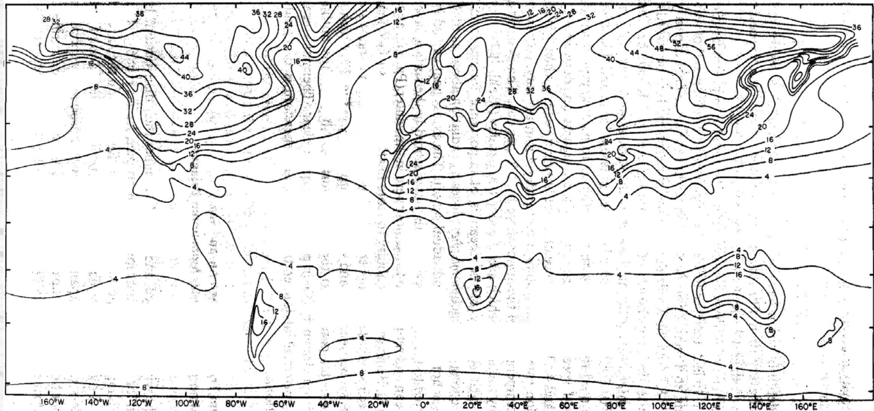
Fig. 2.1. Annual range of monthly mean temperatures at the earth's surface. [Adapted from Mopin (1975, p. 203).]
