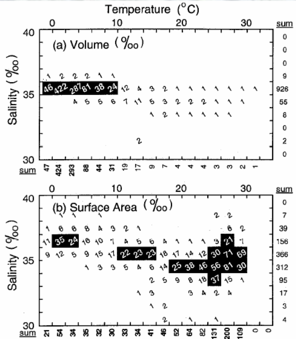
Figure 8. The distribution of the ocean waters as a function of temperature (in degrees Celsius) and salinity (in per mil). The distributions are shown as (a) per mil (i.e., ‰) of
